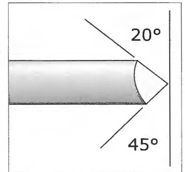
Figure 3: Bowl gouge side view
