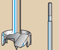
Multi spur bit
